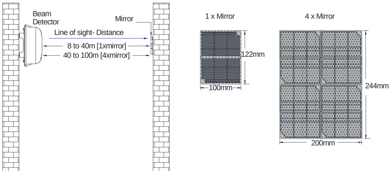
Figure 6: Mounting of TX7130-R Reflector Mirror
